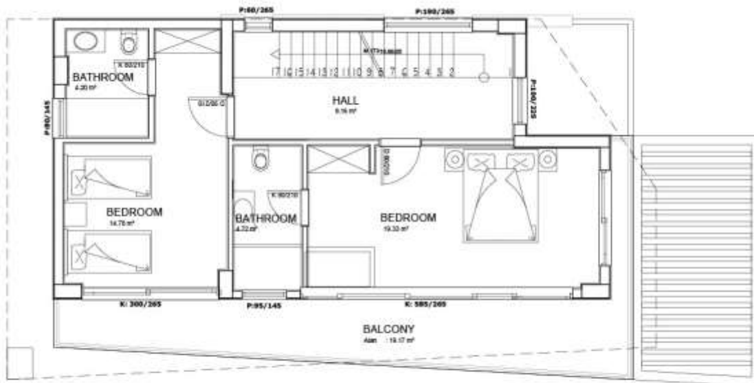
A BLOCK FIRST FLOOR PLAN 82.64 m 2
